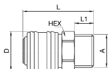
Male Thread
